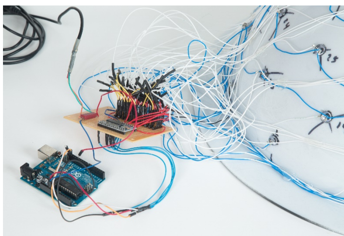
Figure 6. Close-up image of the wiring on the prototype RTI system.
